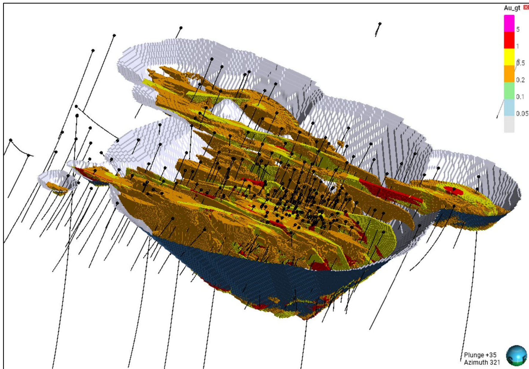
Figure 2 – Overhead 3D Down plunge View looking NW showing Inferred Blocks above the 0.22 g/t Au cut-off grade and inside the Pit Shell
